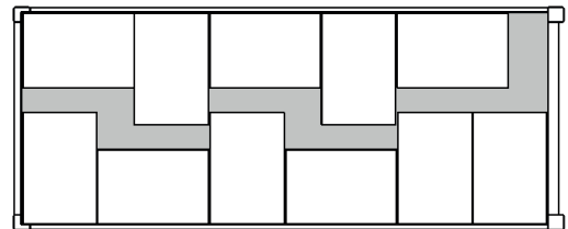
Figure 7.30 – Packing 800 × 1,200 mm unit loads into a 20-foot container
