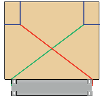
Figure 7.48 – Transverse spring lashing
