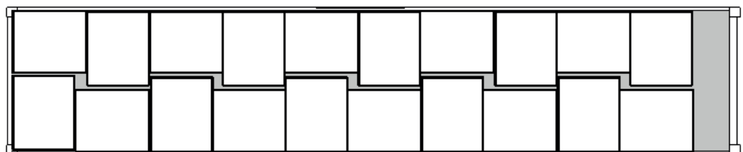
Figure 7.31 – Packing 1,000 × 1,200 mm unit loads into a 40-foot container
