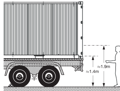
Figure 5.10 – Seal heights – freight container
