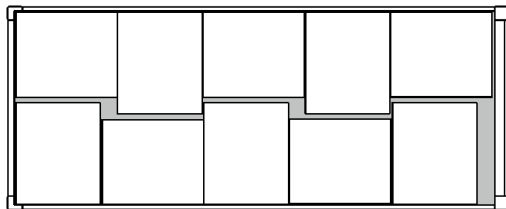
Figure 7.29 – Packing 1,000 × 1,200 mm unit loads into a 20-foot container
