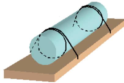
Figure 7.44 – Silly-loop lashing
