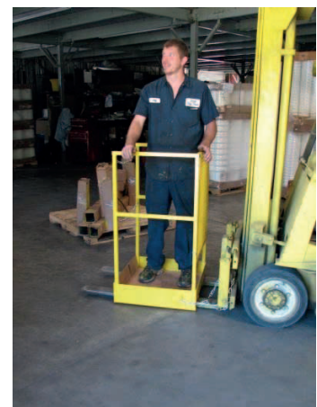
Figure 5.15 – Mobile work station
