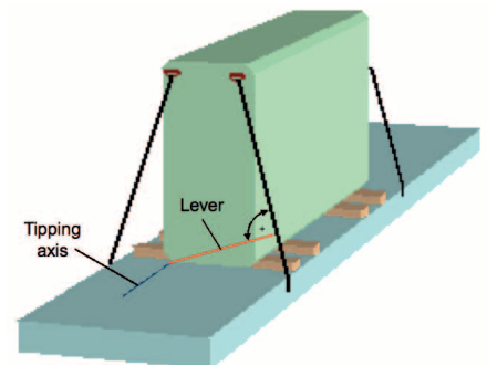
Figure 7.39 – Direct lashing against tipping
