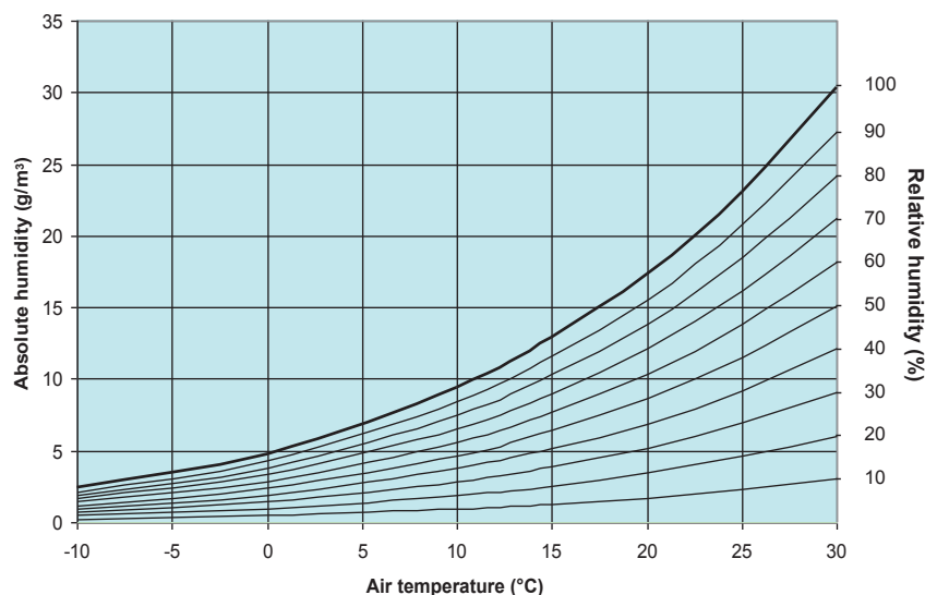
Figure 3.1 – Absolute and relative humidity
