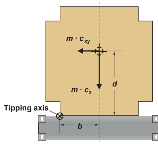
Figure 7.37 – Tipping criterion
