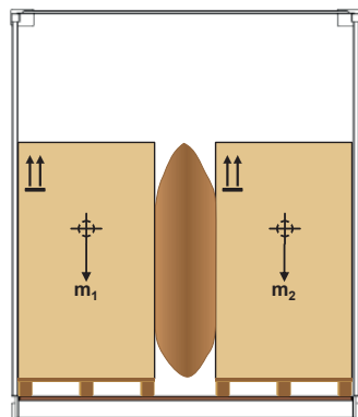
Figure 7.59 – Equal height packages
