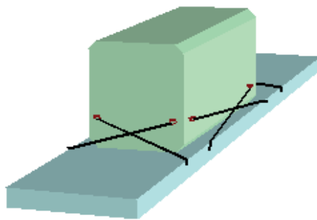
Figure 7.38 – Direct lashing against sliding
