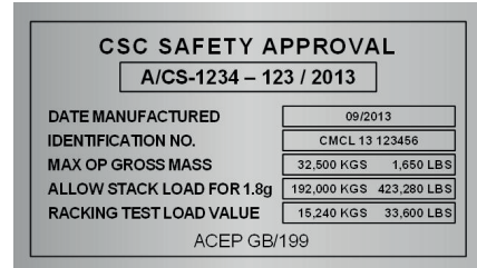
Figure 8.2 – CSC safety approval plate with ACEP mark
