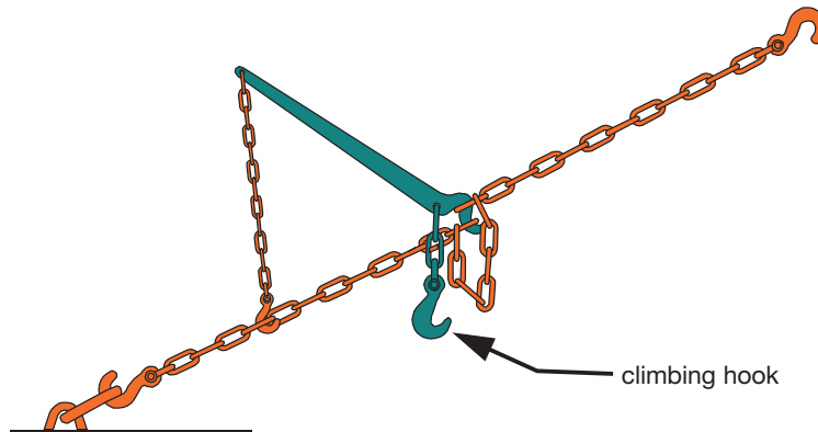
Figure 7.17 – Long link lashing chain with lever tensioner
