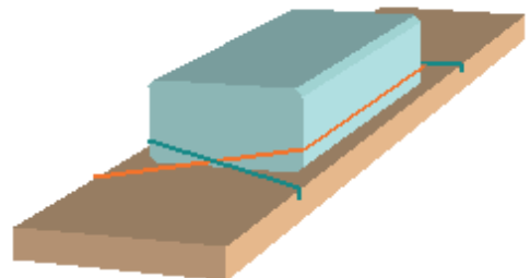
Figure 7.42 – Horizontal half-loop lashing
