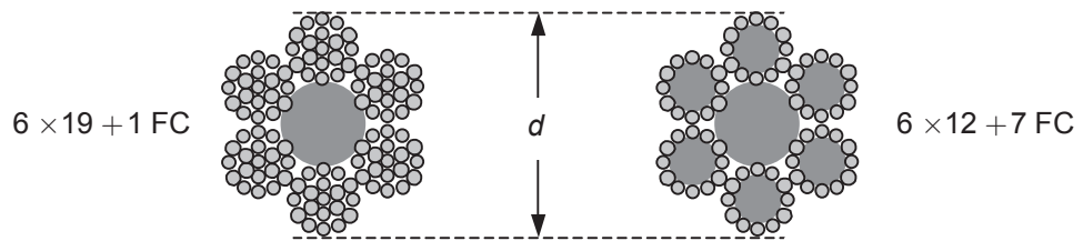
Figure 7.13 – Typical lashing wire rope construction
