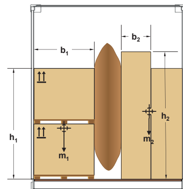
Figure 7.60 – Unequal height packages
