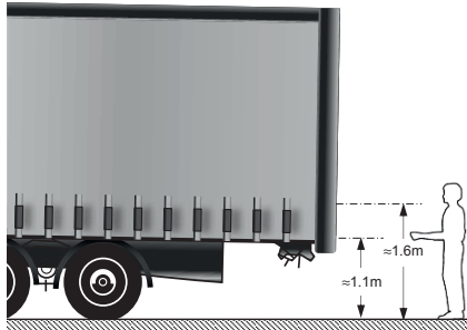
Figure 5.9 – Seal heights – trailer
