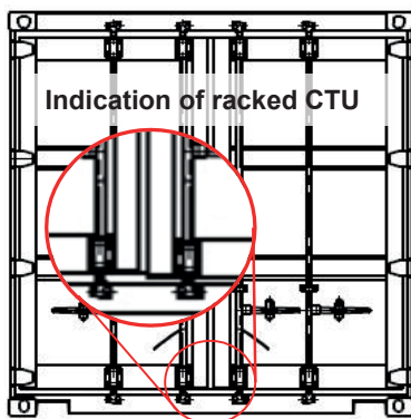
Figure 5.29 – Racked CTU
