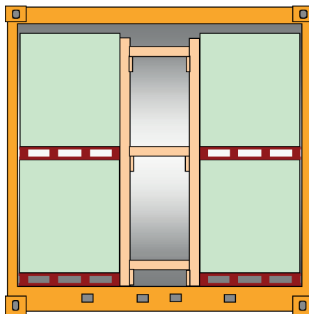
Figure 7.3 – Centre gap with transverse bracing
