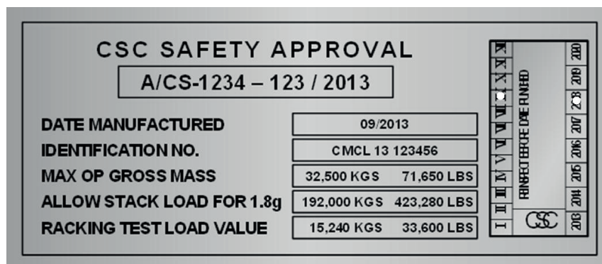
Figure 4.2 – CSC safety approval plate with next examination date
