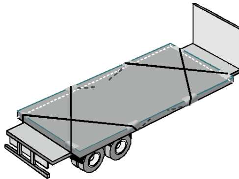
Figure 7.49 – Over-width package secured by half loops
