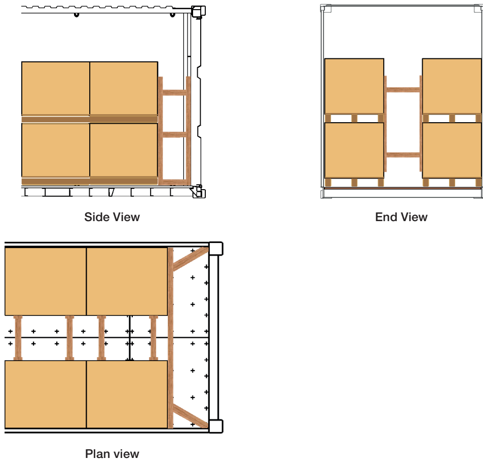
Figure 7.32 – Blocking in a strong boundary CTU
